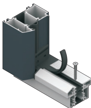
AT 100 D PROFILO DESIGN
